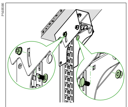
Fix the pendant to the adjustable ceiling plate with 4 bolt sets 22S and align the pendant to the vertical plane before tightening the bolts. Recommended torque 20 N.m.
