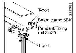
On beams in ceilings, mount Vertical piece 2F as shown in the figure above. When the beam flange thickness does not exceed 13 mm, use Beam clamp 5BK-10 and T-bolt 26U/40. For flange thicknesses not exceeding 30 mm use Beam clamp 5BK-30 and T-bolt 26U/50.
