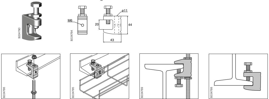
For mounting of Threaded Rod B41 with Flange Nut B43/ M8 – M10.
