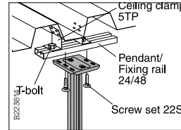
In ceilings with trapezoidal profile sheeting, mount Vertical piece 2FB as shown above
