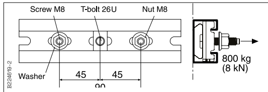
T-bolt 26U M8/M10 + P/F-rail 24/48 + Washer 8.4x19x1.5
