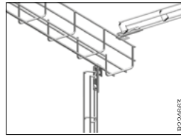
The mounting coupler can be used for vertical and horizontal mounting of Mini Mesh trays onto mesh trays and cable ladders.
