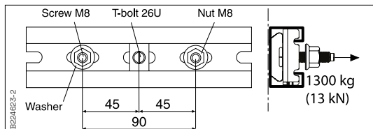
T-bolt 26U M10 + P/F-rail 24/48 + Washer 9x35x2
