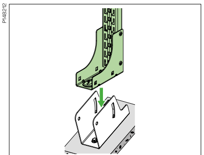
Insert the pendant into the adjustable ceiling plate.
