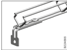
Can be used for mounting of Mini Mesh trays to ceiling, floor and onto wall.
