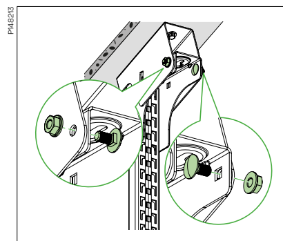
Fix the pendant to the adjustable ceiling plate with 4 bolt sets 22S and align the pendant to the vertical plane before tightening the bolts. Recommended torque 20 N.m.
