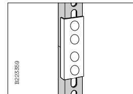
Vertical piece 2F can be joined to achieve the required length using Pendant/fixing rail 24/48 and Pendant joint 2FJ.
