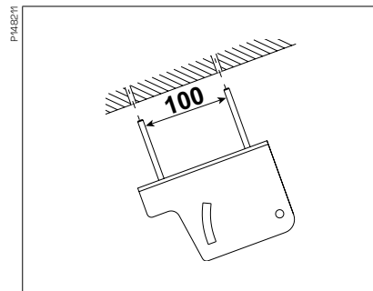
Fix the adjustable ceiling plate to the ceiling with 2 bolts. (c-c: 100 mm).
