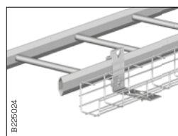
G-Mesh tray mounted on cable ladder, Combi fitting B21 90° is used.
