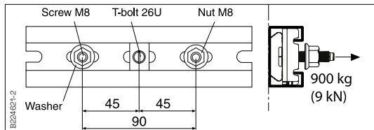
T-bolt 26U M8 + P/F-rail 24/48 + Washer 9x35x2
