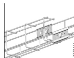
Fittings B1 and B2 are used for joining the mesh trays. Example of joining G-mesh tray with standard mesh tray
