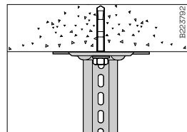
Mount Vertical piece 2F using Expansion bolt alt. Concrete screw.
