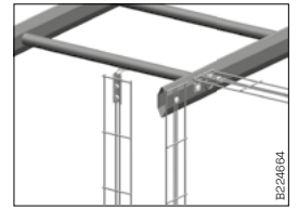
The mounting coupler can be used for vertical and horizontal mounting of Mini Mesh trays onto mesh trays and cable ladders.
